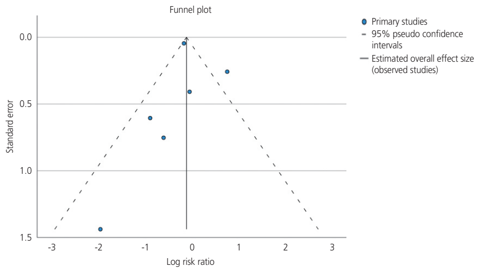
Supplementary Fig. 16. Funnel plot for studies displayed in Supplementary Fig. 15.
