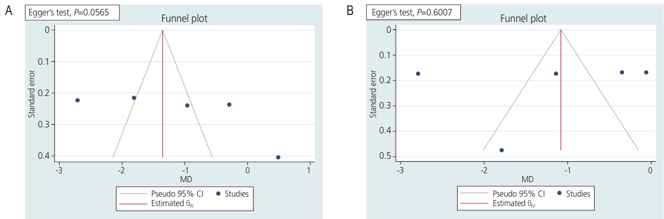
Supplementary Fig. 16. Funnel plots for the mean postoperative pain scores on motion/coughing at 12 (A) and 24 (B) hours. MD, mean difference; CI, confidence interval.
