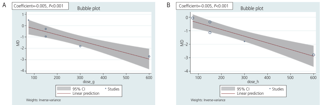
Supplementary Fig. 11. Meta-regression bubble plots for the mean postoperative pain scores on motion/coughing at 12 (A) and 24 (B) hours. MD, mean difference; CI, confidence interval.
